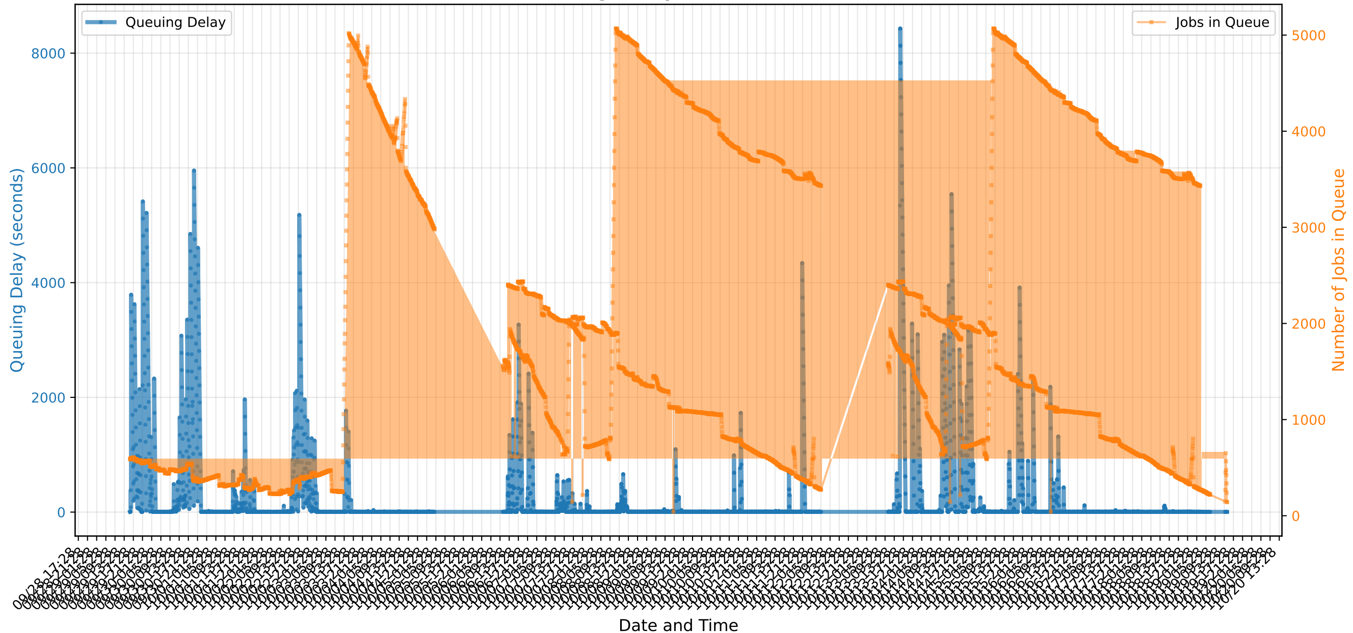
UGE Cluster Queuing Delay Over Time for 16 Core Jobs
